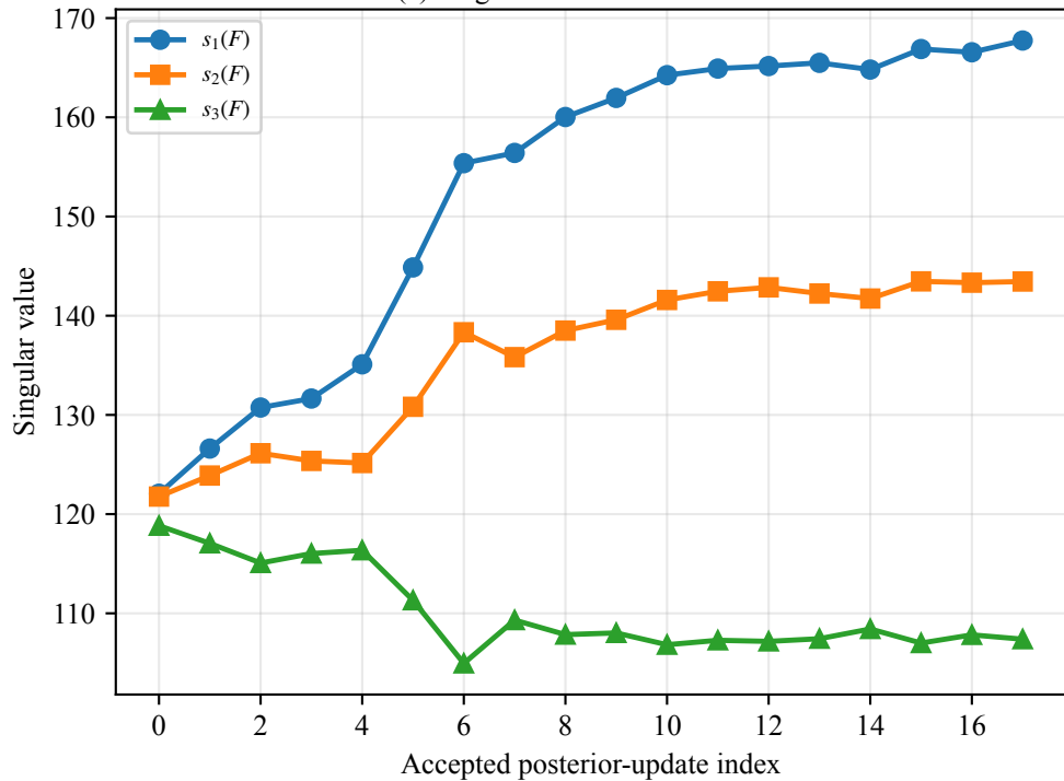
(a) Singular-value evolution of F
